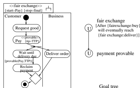
Figure 2: Activity diagram and goal tree
